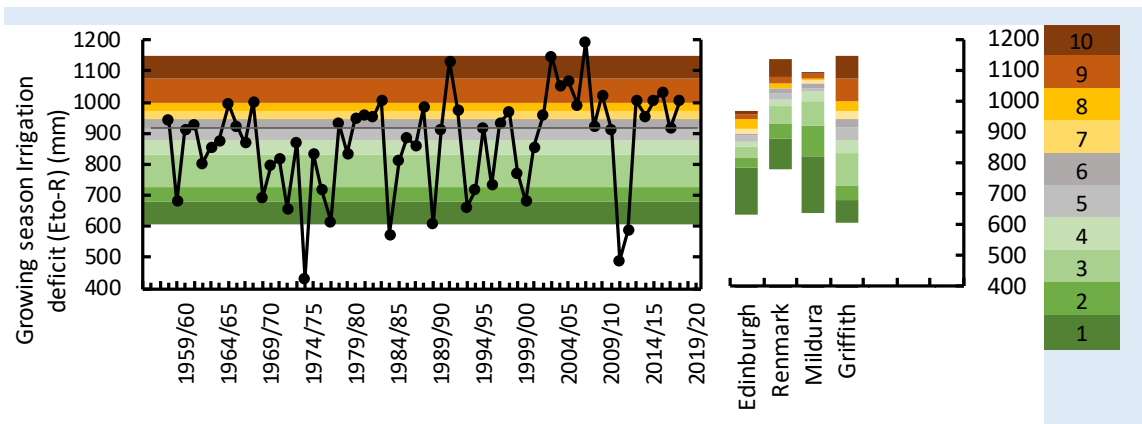
Irrigation demand, measured as the difference between evapotranspiration and rainfall ( ET_o - R ), shows year-to-year variation and an increasing trend in recent decades. 100mm is equivalent to 1ML / ha.
