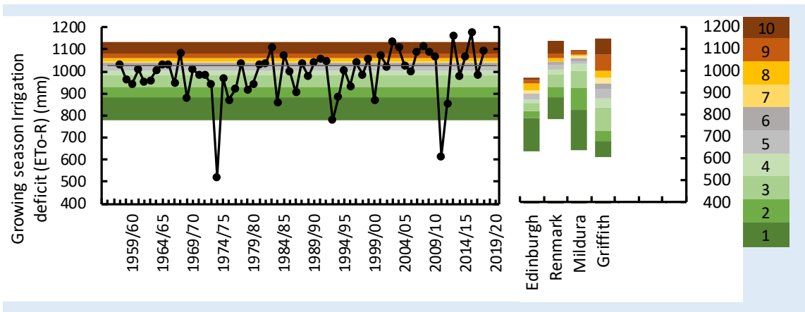
Irrigation demand, measured as the difference between evapotranspiration and rainfall (ETo - R), shows year-to-year variation and an increasing trend in recent decades. 100mm is equivalent to 1ML / ha.
