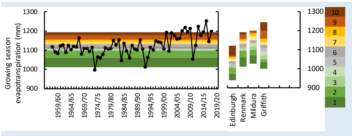
Evapotranspiration (ETo) like rainfall shows year-to-year variation, but unlike rainfall there is a trend of increasing evapotranspiration in recent decades. 100mm is equivalent to 1ML / ha.
