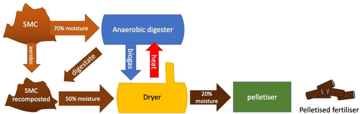
Figure 52. The SmartMushroom process. Derived from www.smartmushroom.eu
