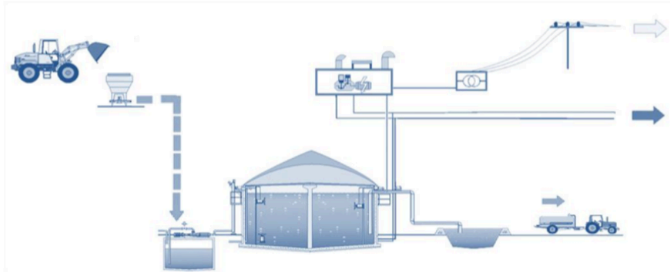
Figure 49. Biogas plant
