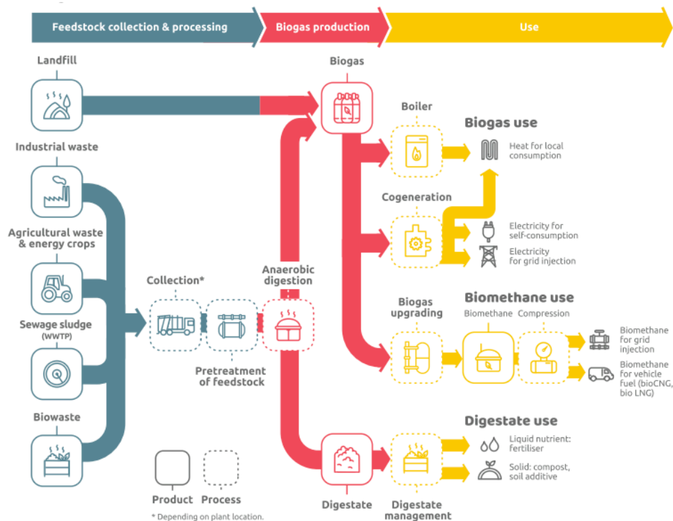
Figure 51. Biogas production. From Carlu et al, 2019.
