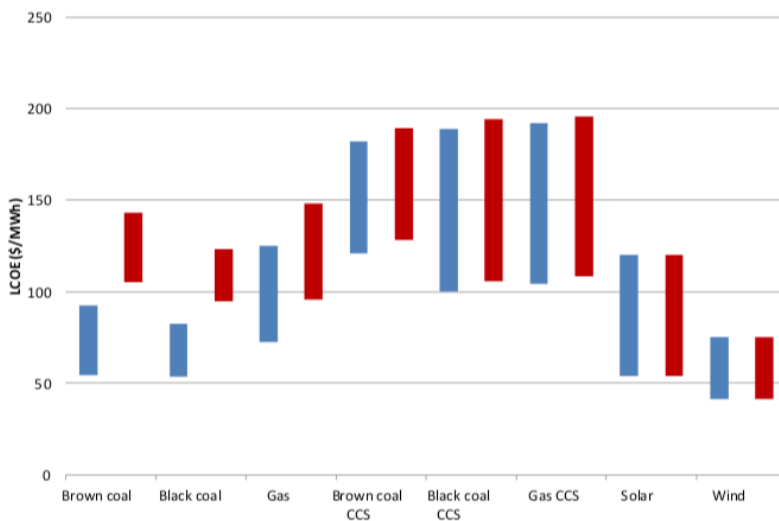
Figure 40. Projected 2030 cost of electricity from different sources with (red) and without (blue) a carbon price. Coal is presented without and with carbon capture and sequestration (CCS) technology. Source: Australian electricity market analysis report.
