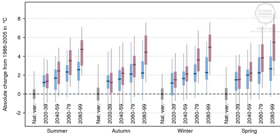
Figure 24. The potential changes in the hottest day (°C) for the Mildura region under a moderate (RCP4.5) and high (RCP8.5) emissions scenario in the four seasons.
