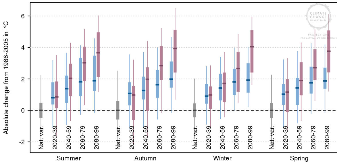
Figure 20. The potential changes in the hottest day (°C) for South East Queensland under a moderate (RCP4.5) and high (RCP8.5) emissions scenario in the four seasons.
