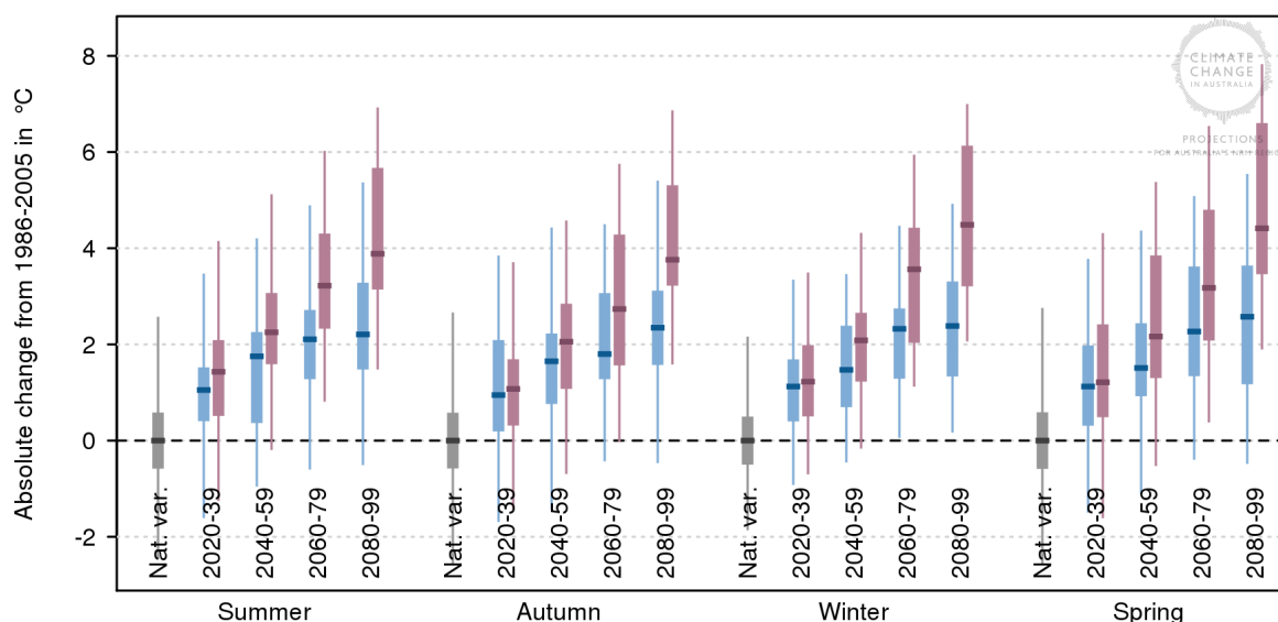
Figure 22. The potential changes in the hottest day (°C) for Sydney and the Hunter valley under a moderate (RCP4.5) and high (RCP8.5) emissions scenario in the four seasons.
