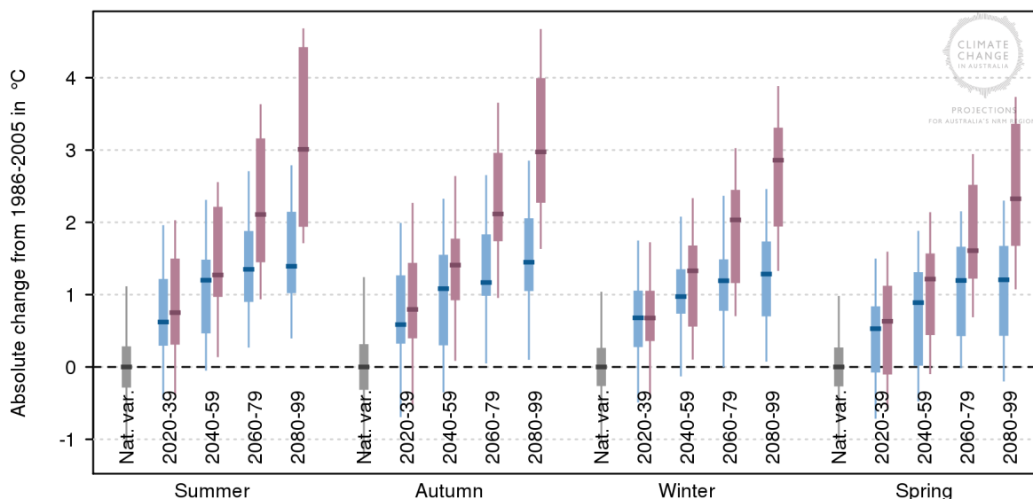
Figure 27. The potential changes in the coldest night (°C) for the Melbourne region under a moderate (RCP4.5) and high (RCP8.5) emissions scenario in the four seasons.
