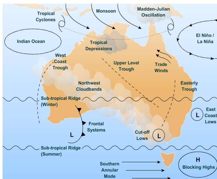
Figure 12. A summary of the family of circulation features that are responsible for much of the climate variability in the short term. (Sources: Climate Change in Australia CSIRO
