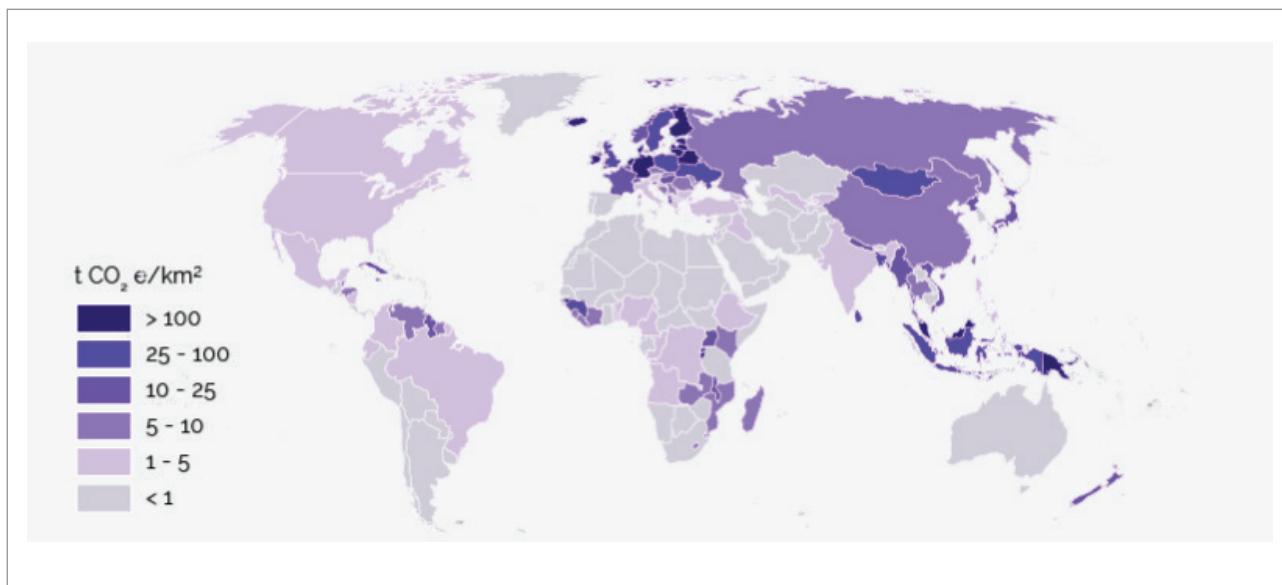
Figure 2. Emissions (tonnes CO 2 /km 2 /year) from drained peatland. Source: Greifswald Mire Center.
