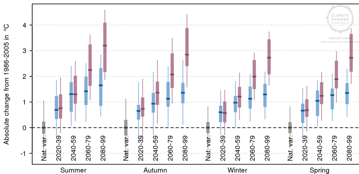
Figure 29. The potential changes in the coldest night (°C) for the Adelaide region under a moderate (RCP4.5) and high (RCP8.5) emissions scenario in the four seasons.
