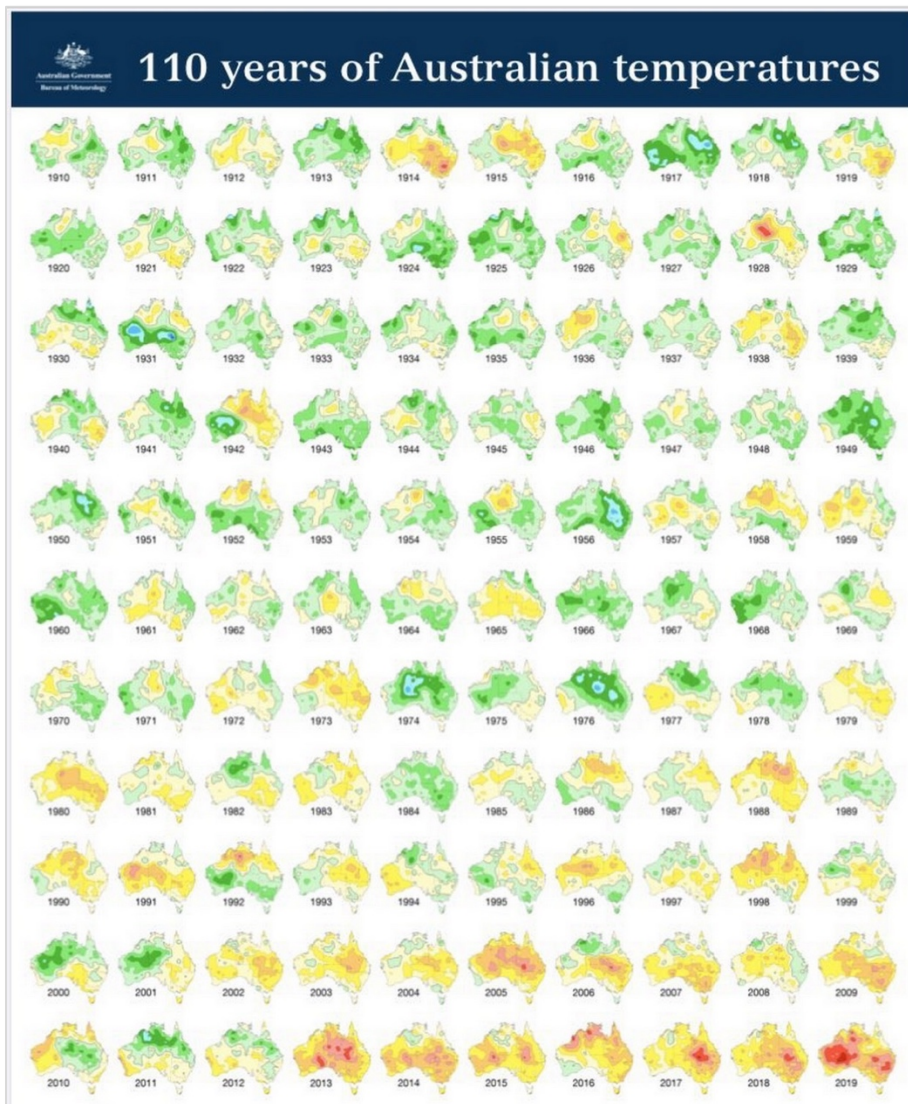
Figure 14. Annual deviations from long term average temperatures. Colours range from dark blue (>3°C below average) to cream (average) to red-brown (>3°C above average)
