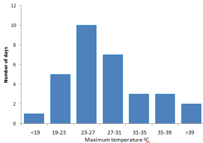
Figure 19. The distribution of daily maximum temperatures for Manjimup during December 2012. The monthly mean was 27.8°C but during December there were 5 days above 35°C.
