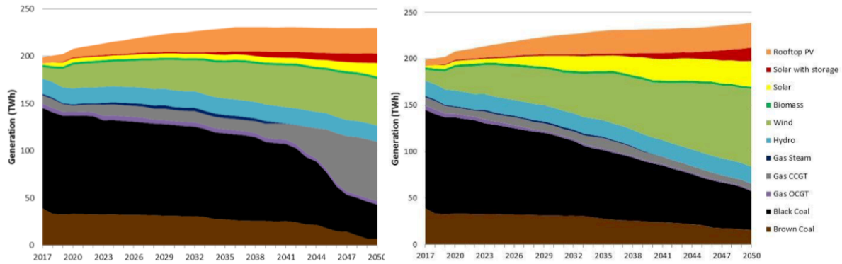
Figure 39. Projected changes in generation type under a business as usual scenario (left) or a clean energy target (right)
