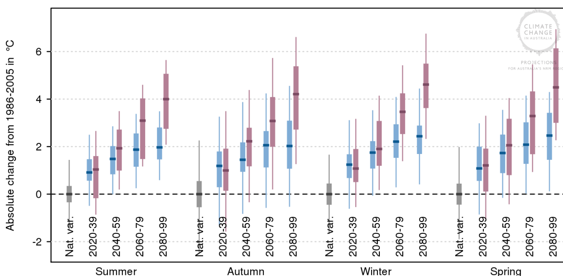
Figure 30. The potential changes in the hottest day (°C) for the Perth region under a moderate (RCP4.5) and high (RCP8.5) emissions scenario in the four seasons.
