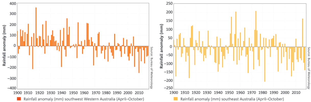
Figure 15. Average rainfall changes in southwestern and south-eastern Australia since 1900 (Source: State of the Climate report 2018)
