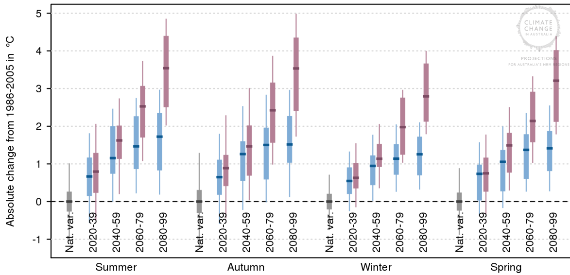
Figure 31. The potential changes in the coldest night (°C) for the Perth region under a moderate (RCP4.5) and high (RCP8.5) emissions scenario in the four seasons.
