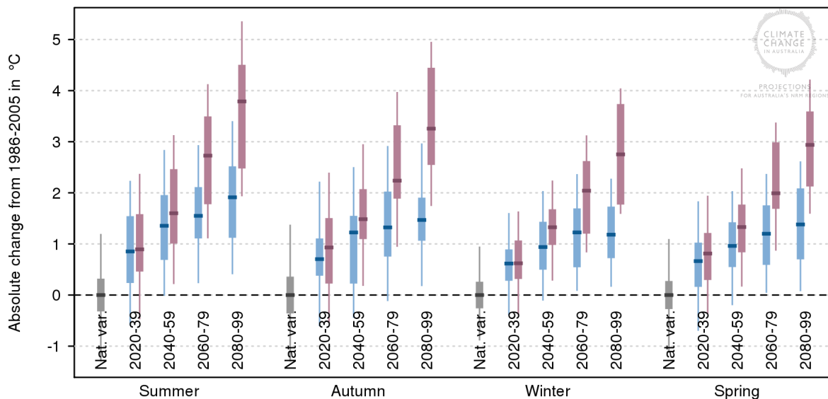
Figure 25. The potential changes in the coldest night (°C) for the Mildura region under a moderate (RCP4.5) and high (RCP8.5) emissions scenario in the four seasons.
