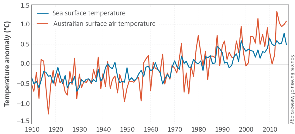
Figure 13 Average air and sea temperature rise since 1910 (Source: State of the Climate report 2018)
