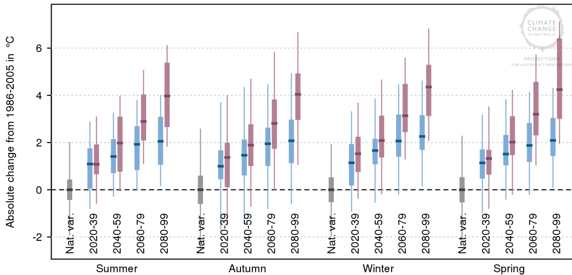
Figure 28. The potential changes in the hottest day (°C) for the Adelaide region under a moderate (RCP4.5) and high (RCP8.5) emissions scenario in the four seasons.
