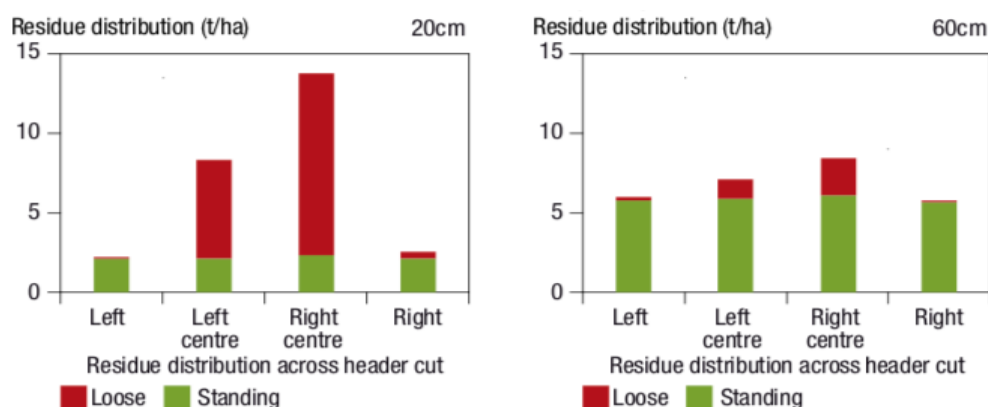
Figure 42. Loose crop residues available for baling when harvesting with 20cm vs 60cm cutting heights. Source: WANTFA
