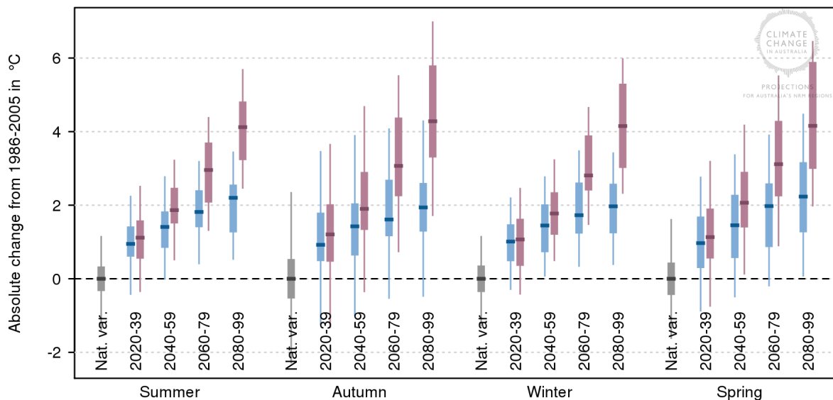
Figure 21. The potential changes in the coldest night (°C) for South East Queensland under a moderate (RCP4.5) and high (RCP8.5) emissions scenario in the four seasons.
