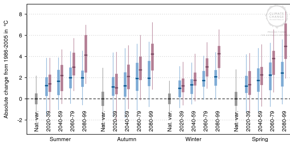
Figure 26. The potential changes in the hottest day (°C) for the Melbourne region under a moderate (RCP4.5) and high (RCP8.5) emissions scenario in the four seasons.
