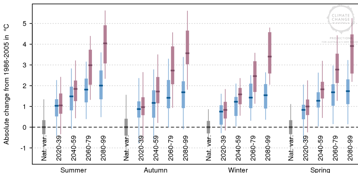
Figure 23. The potential changes in the coldest night (°C) for Sydney and the Hunter valley under a moderate (RCP4.5) and high (RCP8.5) emissions scenario in the four seasons.
