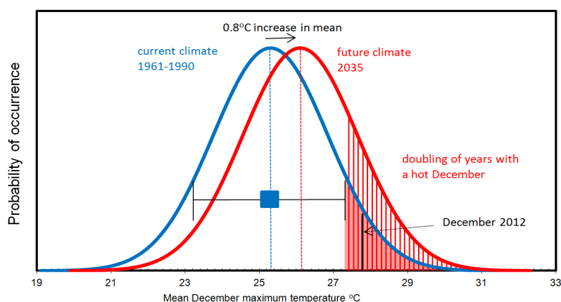
Figure 18. The December mean monthly maximum temperature for Manjimup during 1961-1990 and that projected for 2035.
