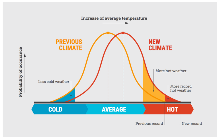
Figure 16 Schematic showing the increased probability of hot extremes and decreased probability of cold extremes with an increase in average temperatures 22 .
