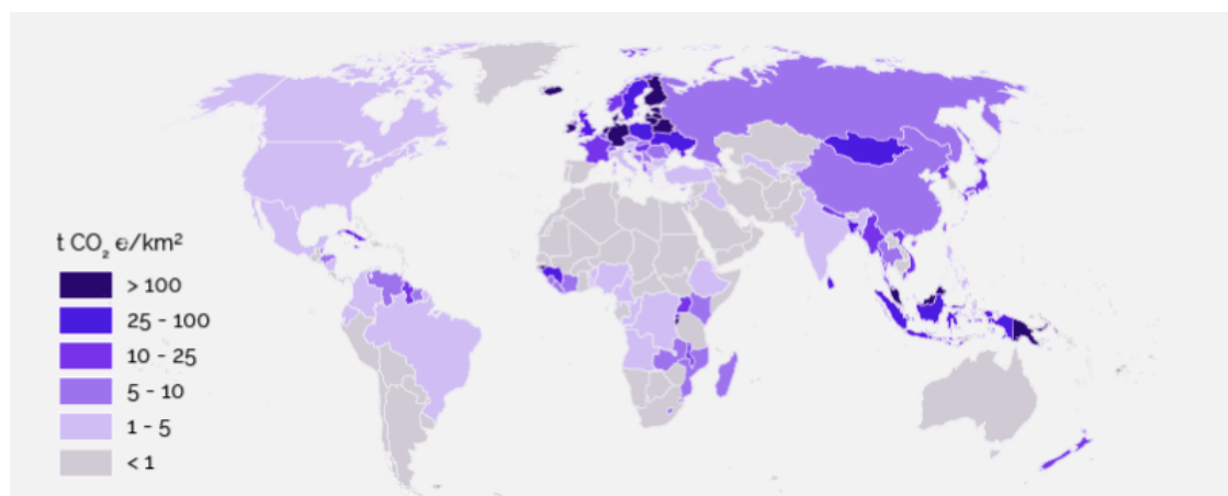
Figure 43. Emissions (tonnes CO 2 /km 2 /year) from drained peatland. Source: Greifswald Mire Center.
